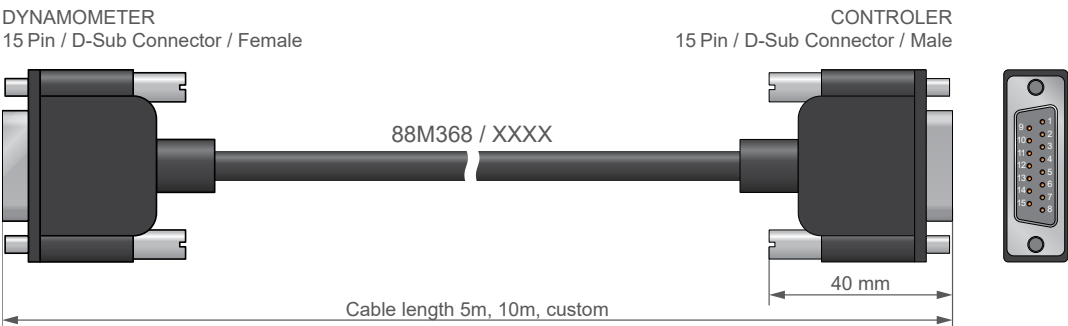
Fig.5-5 Cable 88M368/XXXX - Configuration
