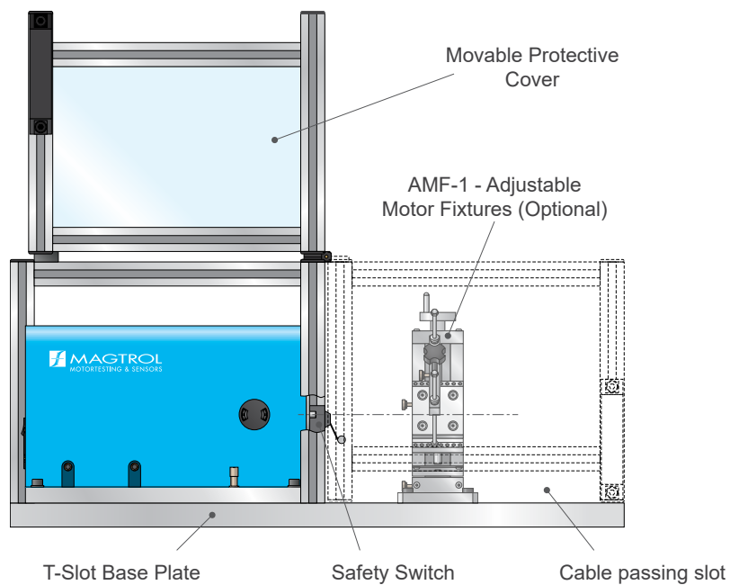
Fig.1-8 "Complete System" version with protective cover
