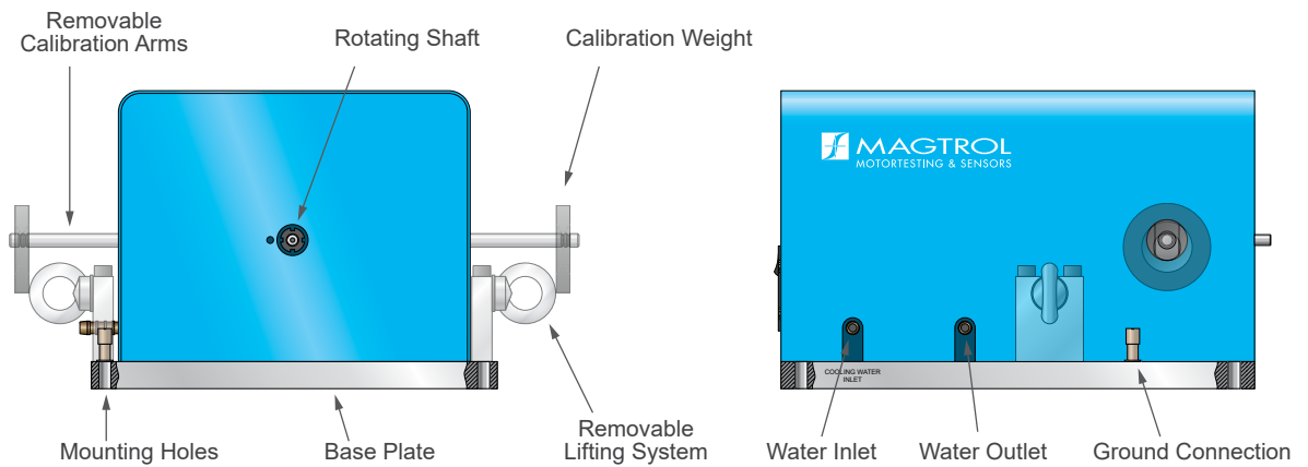
Fig.1-6 Front and left side view
