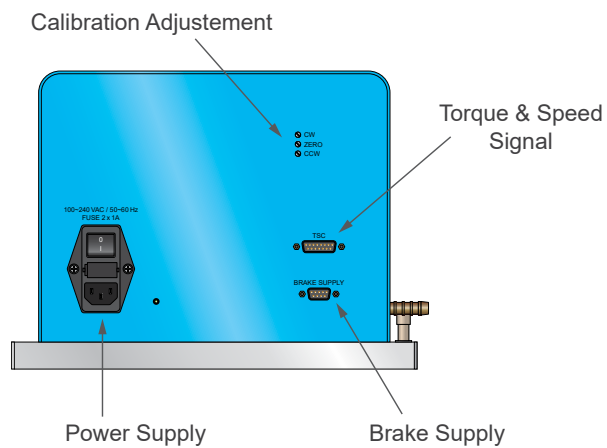
Fig.1-7 Rear view with connection interface
