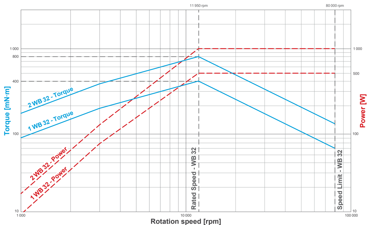
Fig.3-1 WB 32 - Ratings Curves (typical range)
