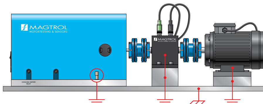
Fig.5-1 Common Earth-grounding
