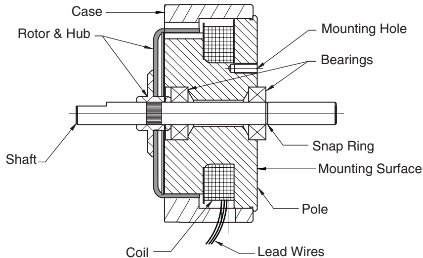
Figure 1. Hysteresis Brake
